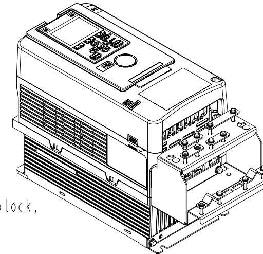
シールドクランプキット取付け完成図 Completed figure after the SHIELD CLAMP KIT has been Installed
